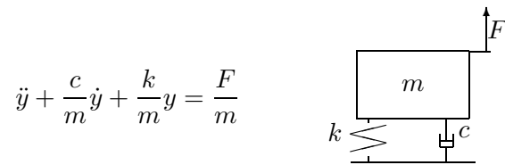
Figure 4: Mass-Spring-Damper System
